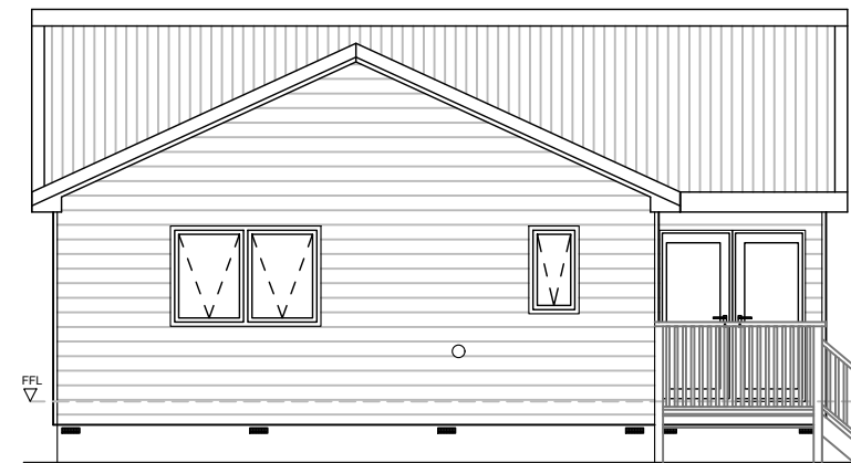
SIDE ELEVATION
